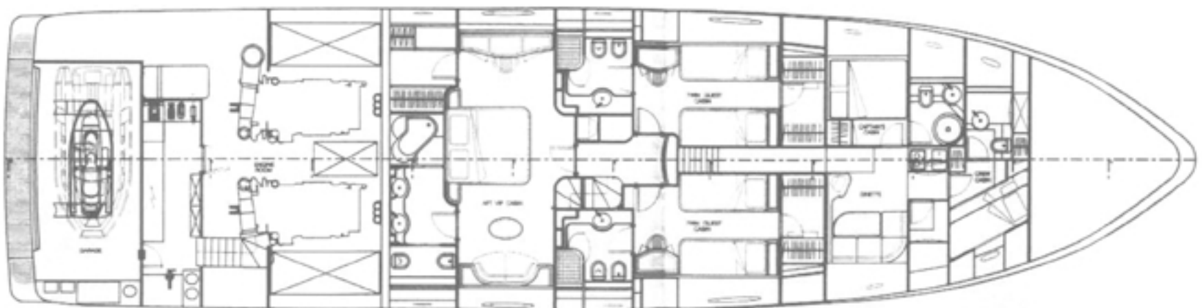
LOWER DECK - CL94' Standard "A"
