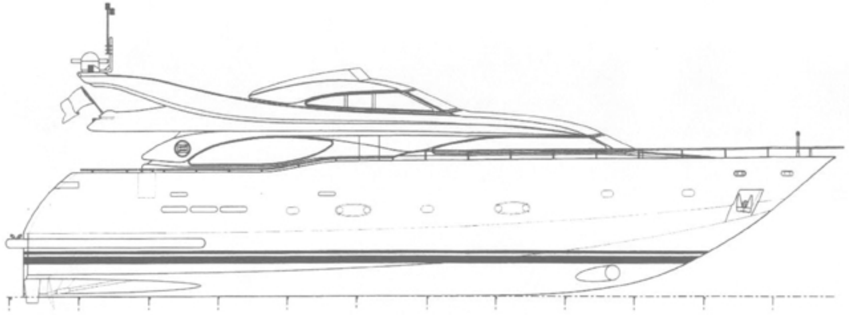
PROFILE - CL94' Standard "A"
